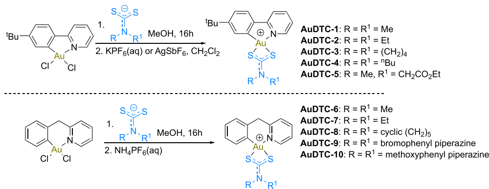
Figure 22. (a) Chemical structures of three-coordinate Au(I), AuTri complexes. (b) Transmission electron microscopy of known cell death inducers, vehicle control, and AuTri-9 in MDA-MB-231. (c) Maximal cristae width. Data are representative of 10 cells chosen at random n = 10 , where mitochondria were also chosen at random. (d) Immunoblots of OPA1, MFF, MFN1, and TOM20. Reproduced from ref 355. Copyright 2021 American Chemical Society.
