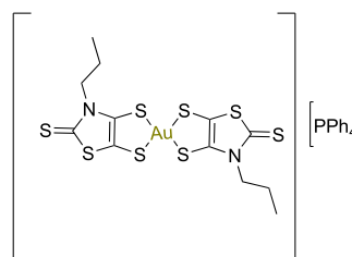
Au(III)-dithiolate-3
