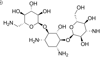
Chart 23. Chemical Structure of Cyclometalated Au(III) Complexes and Kanamycin with Their Bactericidal Activity
