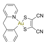
Au(III)-dithiolate-1
