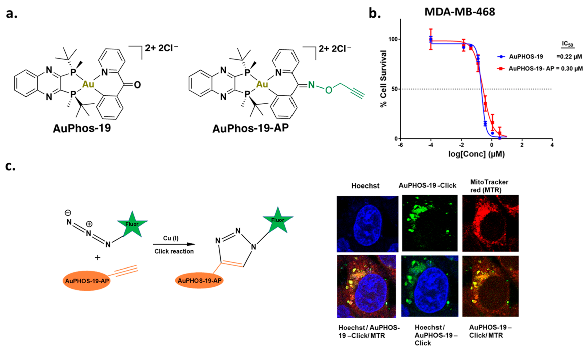
Figure 10. (a) P -chirogenic Au(III) molecule (AuPhos-19) and the alkyne functionalized probe (AuPhos-19-AP). (b) Assessment of cell viability in MDA-468 cells treated with parent molecule (AuPhos-19) versus AuPhos-19-AP. (c) Representation and result of biorthogonal Cu(I)-catalyzed azide–alkyne cycloaddition (CuAAC) reaction using an azide-tagged FITC fluorophore. Reproduced with permission from ref 175. Copyright 2022 Elsevier.
