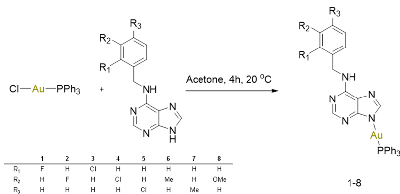
Chart 32. Synthetic Scheme and Structures of Gold Complexes Investigated for Anti-inflammatory Effects in Several Cancer Cell Lines
