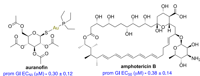
Chart 24. Chemical Structures and Antileishmanial Activity of Auranofin and Amphotericin B
