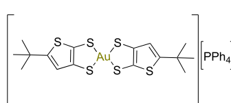
Au(III)-dithiolate-6
