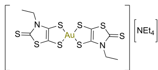
Au(III)-dithiolate-2
