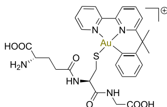
Chart 23. Chemical Structure of Cyclometalated Au(III) Complexes and Kanamycin with Their Bactericidal Activity
