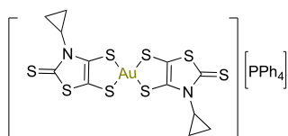
Au(III)-dithiolate-5
