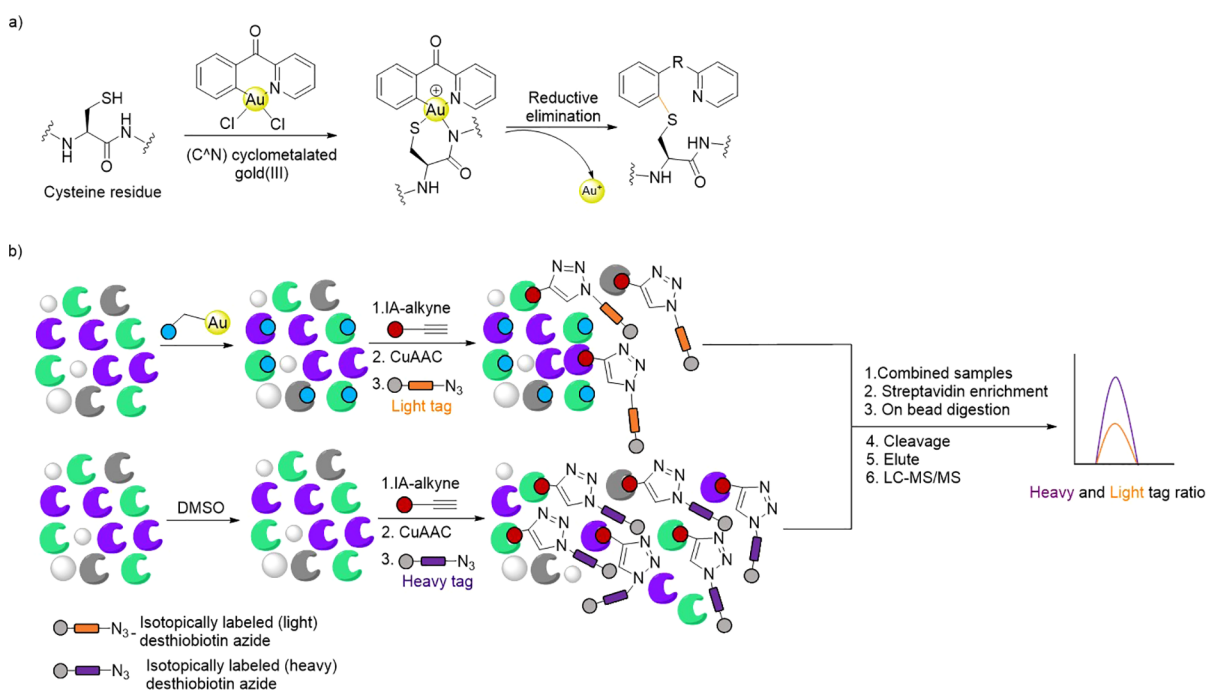
Figure 11. (a) Mechanism of cysteine arylation via Au(III) complex reductive elimination. (b) Workflow of isotopically labeled desthiobiotin activity based protein profiling (isoDTB-ABPP). Figure reproduced from ref 180. Copyright 2022 Royal Society of Chemistry.
