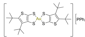
Au(III)-dithiolate-7
